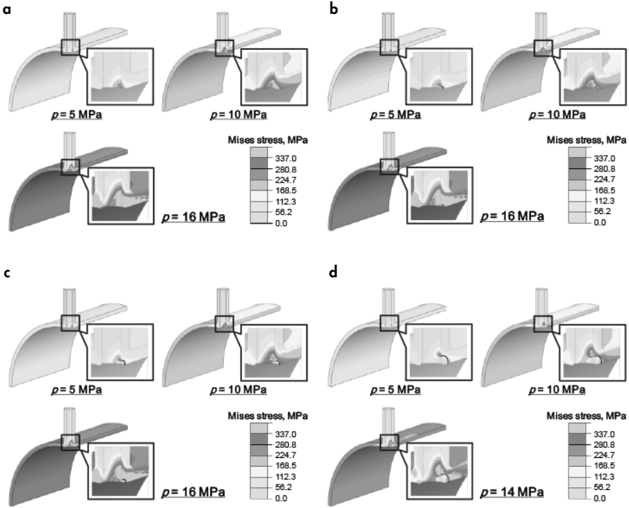
FIG. 5. — von Mises stress contours around the nozzle crotch corner due to internal pressure. a. Non-flawed model. b. Flawed model with a = 20 mm ( a/t_n = 0.09 ). c. Flawed model with a = 40 mm ( a/t_n = 0.19 ). d. Flawed model with a = 100 mm ( a/t_n = 0.47 ).
