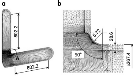
FIG. 3. — Examples of mesh division of T-joint pipes with local wall thinning. a. T-joint quarter model. b. An enlarged view of the eroded area (A)
