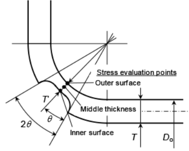
FIG. 4. — Schematic of stress evaluation points at local wall thinning.
