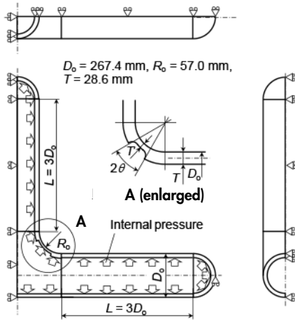
FIG. 1. — Geometry and boundary condition of the T-joint pipe.
