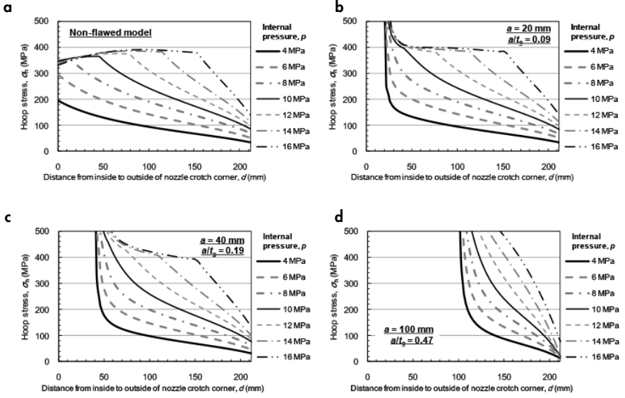
FIG. 6. — Hoop stress distributions from inside through outside of the nozzle crotch corner due to internal pressure. a . Non-flawed model. b . Flawed model with a = 20 mm ( a/t_c = 0.09 ). c . Flawed model with a = 40 mm ( a/t_c = 0.19 ). d . Flawed model with a = 100 mm ( a/t_c = 0.47 ).
