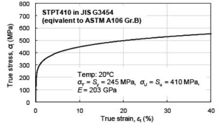
FIG. 2. — Stress-strain curve of STPT410 for FEA.
