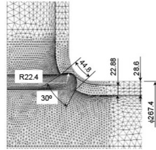
FIG. 8. — Geometry of local wall thinning with T'/T = 0.2 and 2\theta = 30^\circ .
