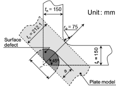
FIG. 3. — Definition of defect geometry at the nozzle crotch corner.
