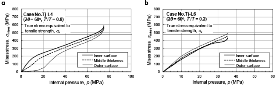
FIG. 5. — Examples of relationship between von Mises stress and internal pressure. a. 2\theta = 60^\circ , T'/T = 0.8 . b. 2\theta = 60^\circ , T'/T = 0.2 .
