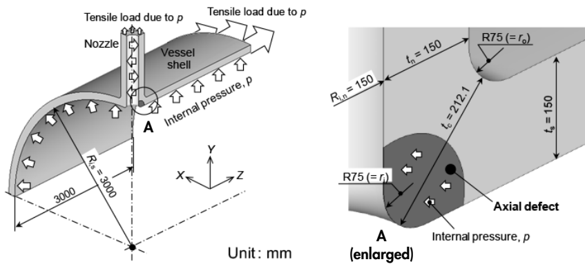
FIG. 2. — 3D model of the nozzle crotch corner in a pressure vessel.
