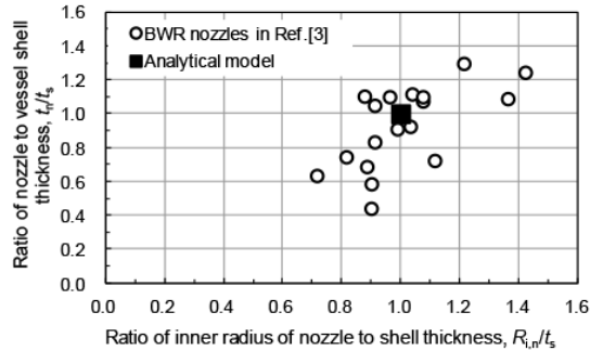
FIG. 1. — Nozzle geometries of BWR nozzles and analytical model.
