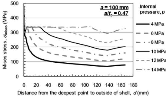
FIG. 8. — von Mises stress distribution from the deepest point to outside evaluation point at collapse section for flawed model with a = 100 mm ( a/t_c = 0.47 ).
