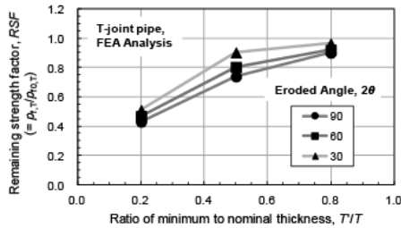
FIG. 6. — Effect of local wall thinning geometry on failure pressure of T-joint pipes.
