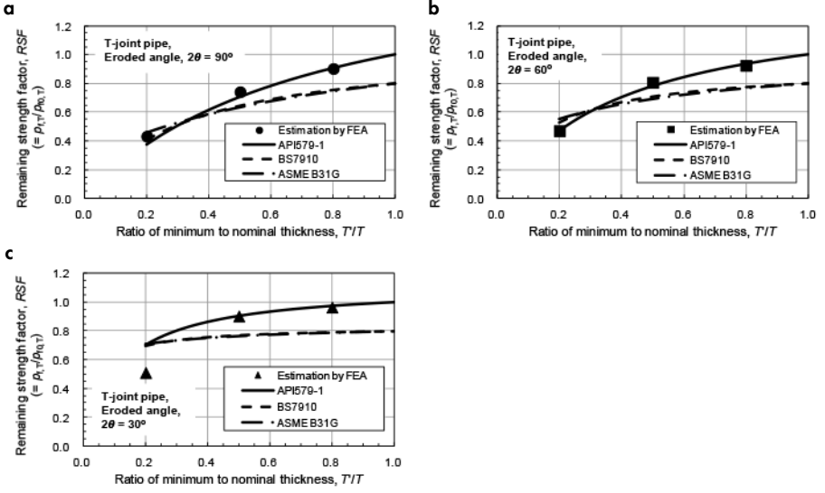
FIG. 7. — Comparison of remaining strength factor for T-joint pipes estimated by FEA and acceptance standards in several fitness-for-service codes. a. 2\theta = 90^\circ . b. 2\theta = 60^\circ . c. 2\theta = 30^\circ .
