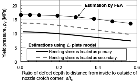
FIG. 9. — Comparison of yield pressures p_Y estimated from L_r parameter for plate model and FEA.
