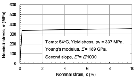
FIG. 4. — Assumed stress-strain curve for application of elastic-plastic FEA.
