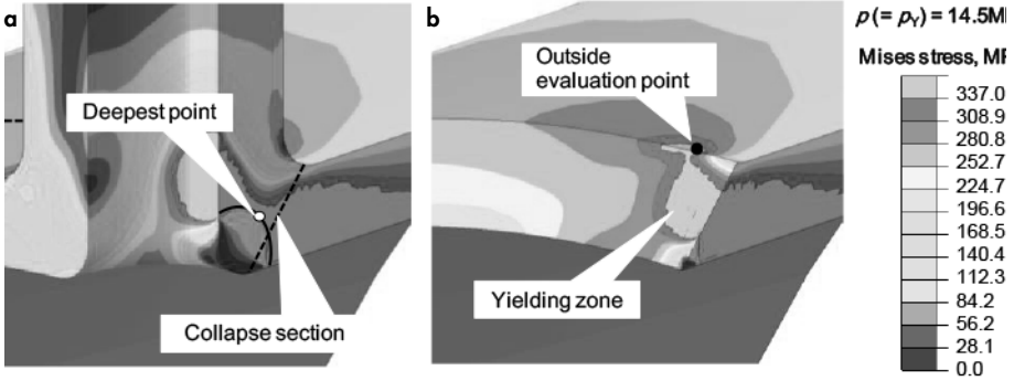
FIG. 7. — von Mises stress contours at the yield pressure p_Y for a deep flawed model with a = 100 mm ( a/t_c = 0.47 ). a. Nozzle corner region. b. Nozzle cutting model at the collapsed section.
